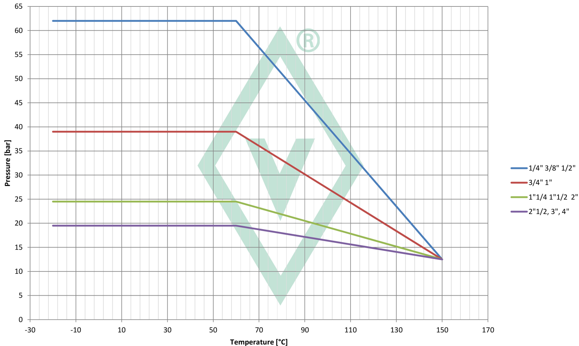
Pressure/Temperature Chart
