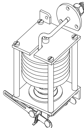
Complete Low Pressure Element
